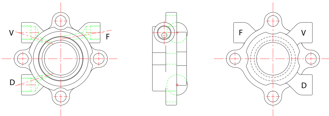
FLUSH-VENT-DRAIN GLAND, TAKES FLEX MOUNT TYPE MECHANICAL SEAL SEAT WITH O-RING.
